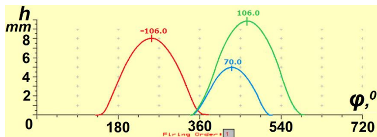
Figure 7. The valve timing for the calculation in Lotus Engine Simulation software: the mode with a lowered lift and reduced opening timing of one of the intake valves.
