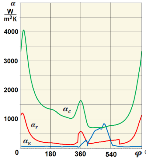
Figure 12. The calculated change in the instantaneous heat transfer coefficient over the cycle at n=6000 rpm with the full opening of the intake valve (head temperature is 660K).
