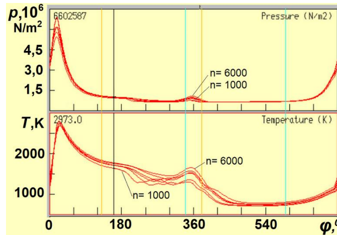
Figure 8. Pressure and temperature change of the gas in cylinder calculated by crank angle within the diapason of the rotation speed of 1000-6000 rpm for the event when both valves are opened simultaneously.
