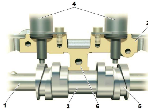
Figure 4. The scheme of the variable intake timing mechanism in the analysed engine: 1- camshaft, 2- frame, 3- sliding cam element mounted on the splines, 4- adjuster magnets, 5- groove for the axial displacement of the cam element, 6- axial bearing.
