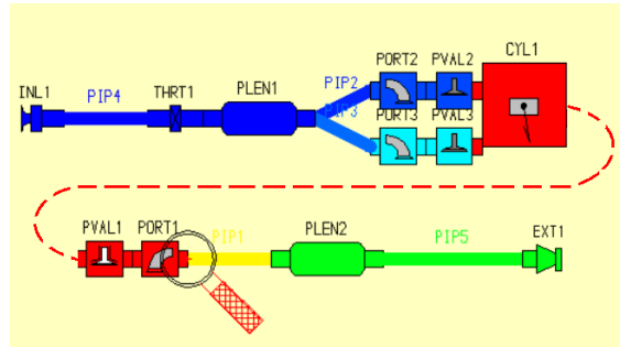
Figure 6. A one-cylinder geometrical model of the engine in the Lotus Engine Simulation software with the means of setting various lifts and phases of the intake valves.
