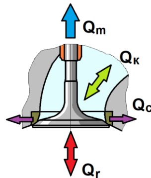
Figure 10. Thermal calculation model of the intake valve.
