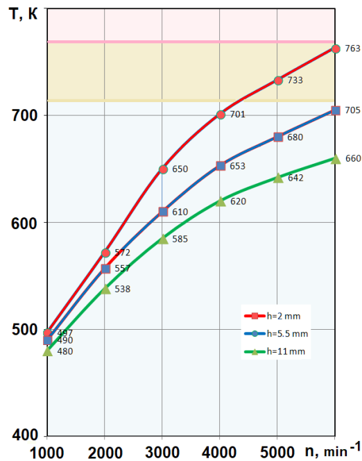
Figure13. The dependence of the temperature of the intake valve on its lift (and the opening duration) with increasing rotation speed.
