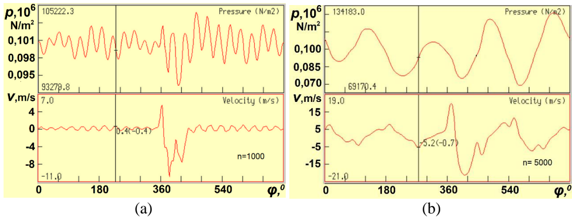
Figure 11. Oscillation of pressure and air velocity by the crank rotation angle in the intake pipe at a distance of 30 mm from the closed valve at (a) 1000 rpm and (b) 5000 rpm.
