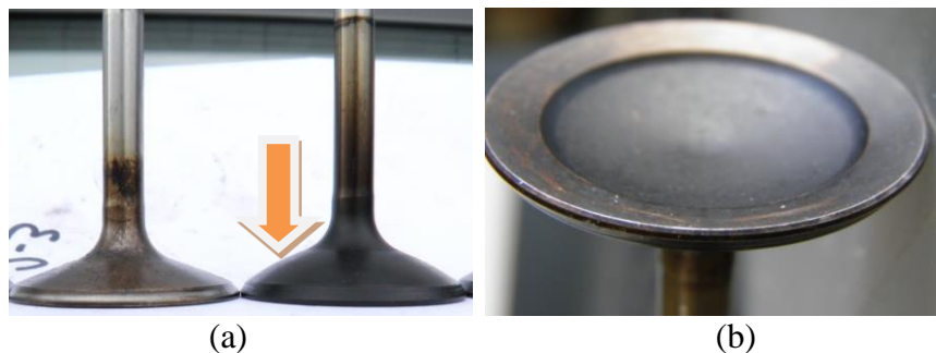
Figure 1. Head deformation of one of the intake valves (a) in the “tulip” shape of a “tulip” with the adjacent intake valve in the same cylinder having taken no damage (b), has no distinct explanation in the common list of causes of thermal overload of the valves including the combustion process failure.
