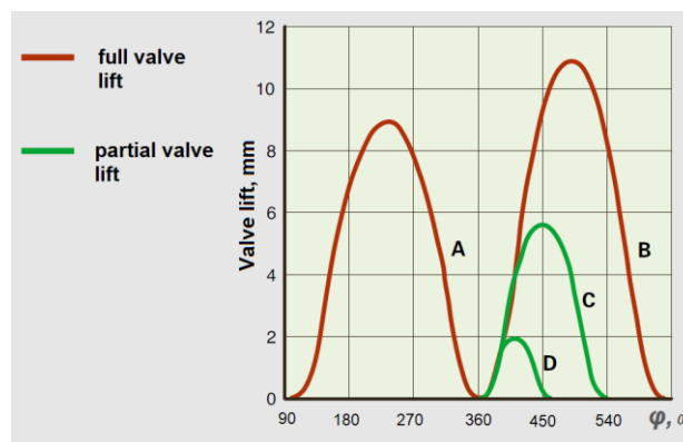
Figure 5. Variable valve timing control program of the analysed engine (full stroke line, partial stroke line, valve stroke in mm with respect to the crank angle in °).
