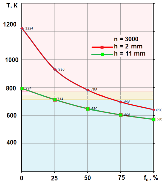
Figure 14. According to the simulation results, the intake valve with a minimum lift ( h=2 mm) overheat even at a small loss of the contact area with the seat (specified by the relative contact area f_c ).
