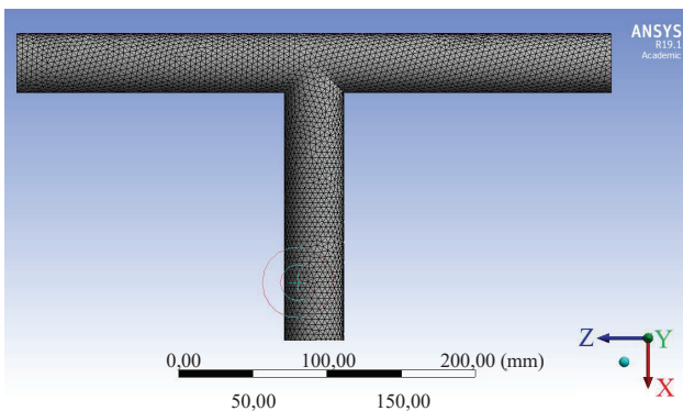
Fig. 2. The finite-volume model of the flow area with a side outlet at 90^\circ
