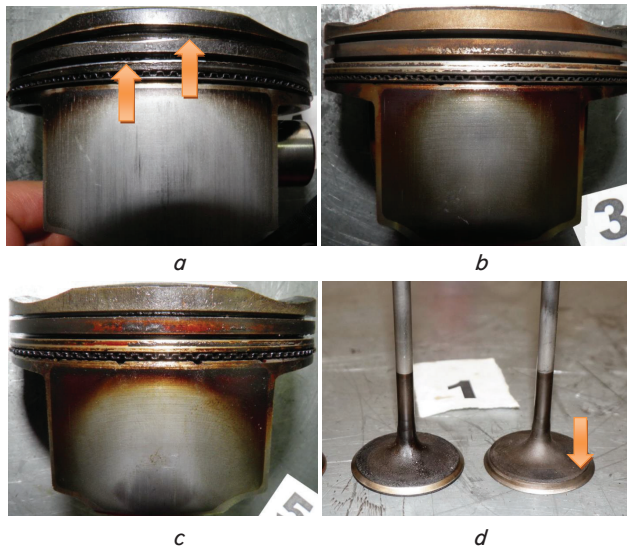
Fig. 11. V6 engine pistons and valves with an intake manifold shown in Fig. 10 after the operation with a non-regular air filter: a – piston No. 1 (arrows show the extremely worn grooves of rings); b – piston No. 3; c – piston No. 5; d – valves of cylinder No. 1 (an arrow shows a heavily worn valve, located further from the inlet to the intake manifold)
