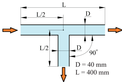
Fig. 1. The geometry of a channel with a side outlet at angle 90^\circ – the length L and the diameter D are assigned
