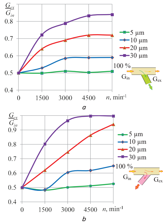
Fig. 8. The results of the simulation of a two-phase flow in a channel with a side outlet at an angle: a - 45^\circ ; b - 135^\circ
