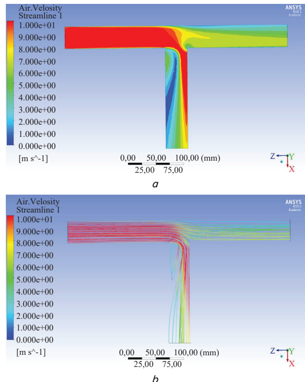
Fig. 3. Results of the refined calculation of the flow of air in a branching channel at angle 90^\circ : a – the field of flow velocities, b – the flow streamlines
