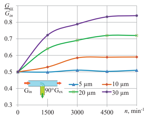
Fig. 5. The results of the simulation of a two-phase flow of air with dust in a channel with a side outlet at an angle of 90°
