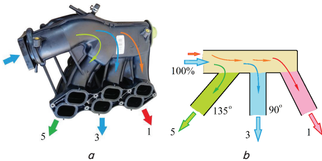
Fig. 9. The ICE intake manifold with different offtake angles (digits 1, 3, and 5 are the numbers of the engine cylinders): a – structural execution; b – estimation scheme of the channels’ offtake angles
