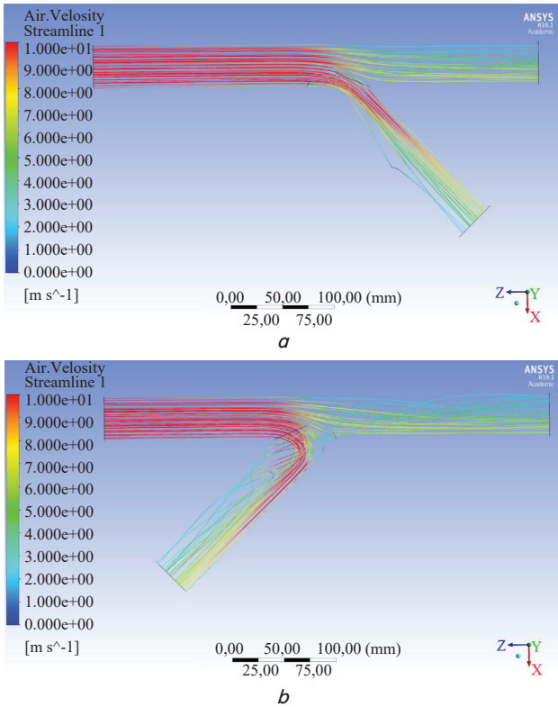
Fig. 6. Streamlines and air velocity streamlines (at a 10 m/s rate at the inlet) in a channel with a side outlet at an angle: a - 45^\circ , b - 135^\circ
