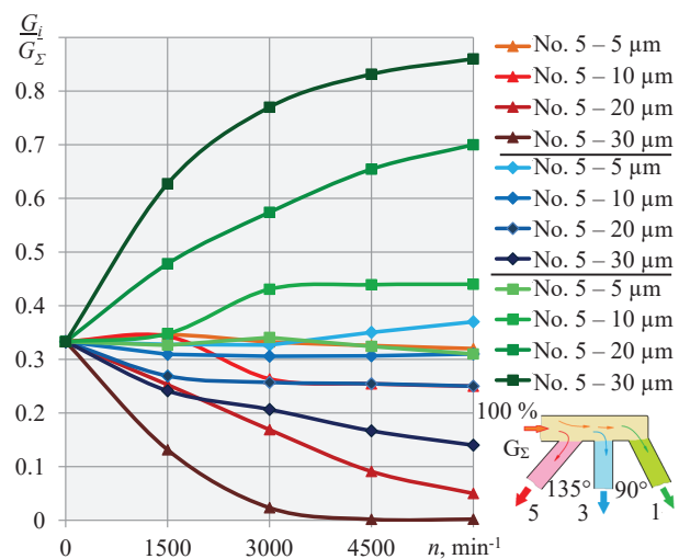
Fig. 10. The ratio of the number of dust particles G_i the size of 5, 10, 20, and 30 \mu\text{m} in the cylinders to the total number of particles G_\Sigma at the inlet at different rotation frequency n of the crankshaft
