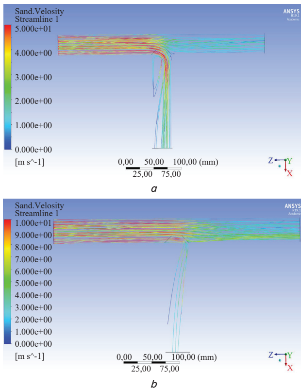
Fig. 4. The trajectories and velocity of dust particles in a branching channel at angle 90°: a – particles of 5 μm, which move at the inlet at a rate of 5 m/s; b – 30 μm particles that move at the inlet at a rate of 15 m/s
